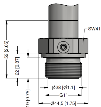
G1" flush (DIN 3852)
